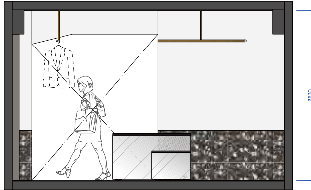
ELEVATION_D-D
